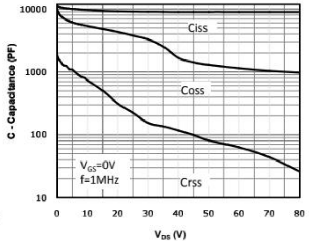
Fig 6: Capacitance Characteristics
