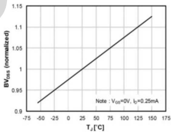
Fig 6. Breakdown Voltage with Temperature
