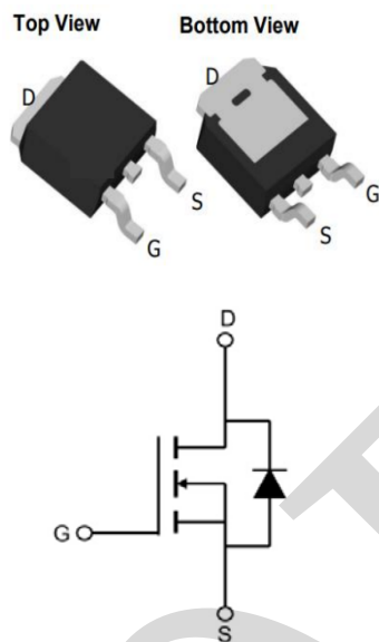
MCR65B580D TO-252
