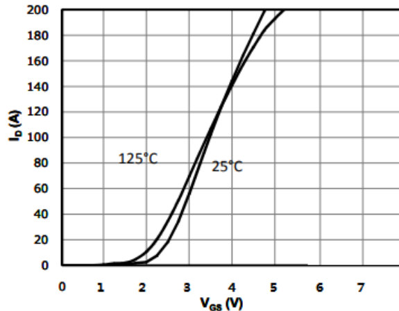
Fig 2: Transfer Characteristics
