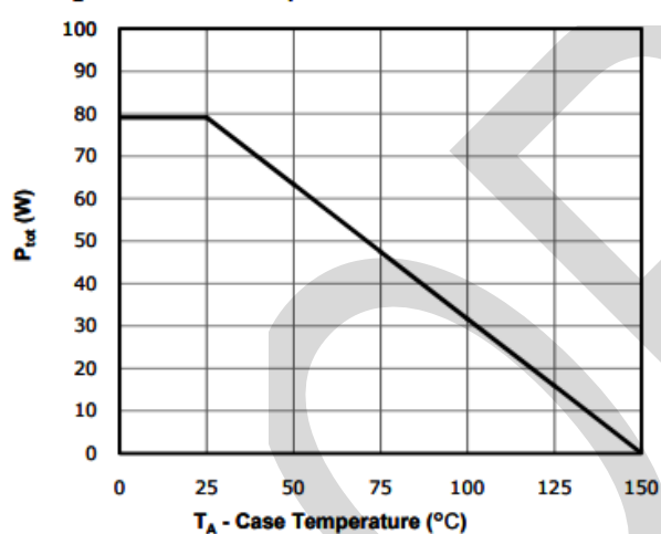
Fig 9: Power Dissipation
